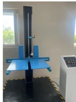
Drop test machine
