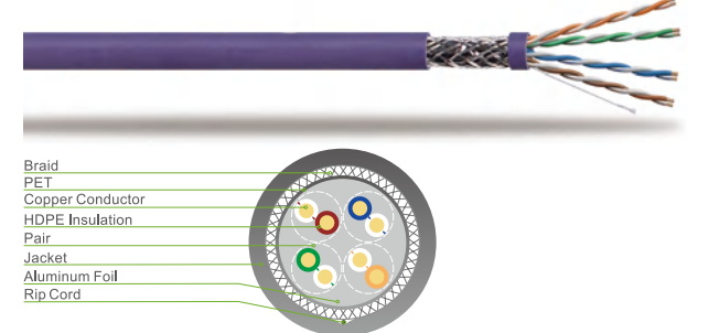
S/FTP Double Fully Shielded CAT 5e Twisted Pair Installation Cable
