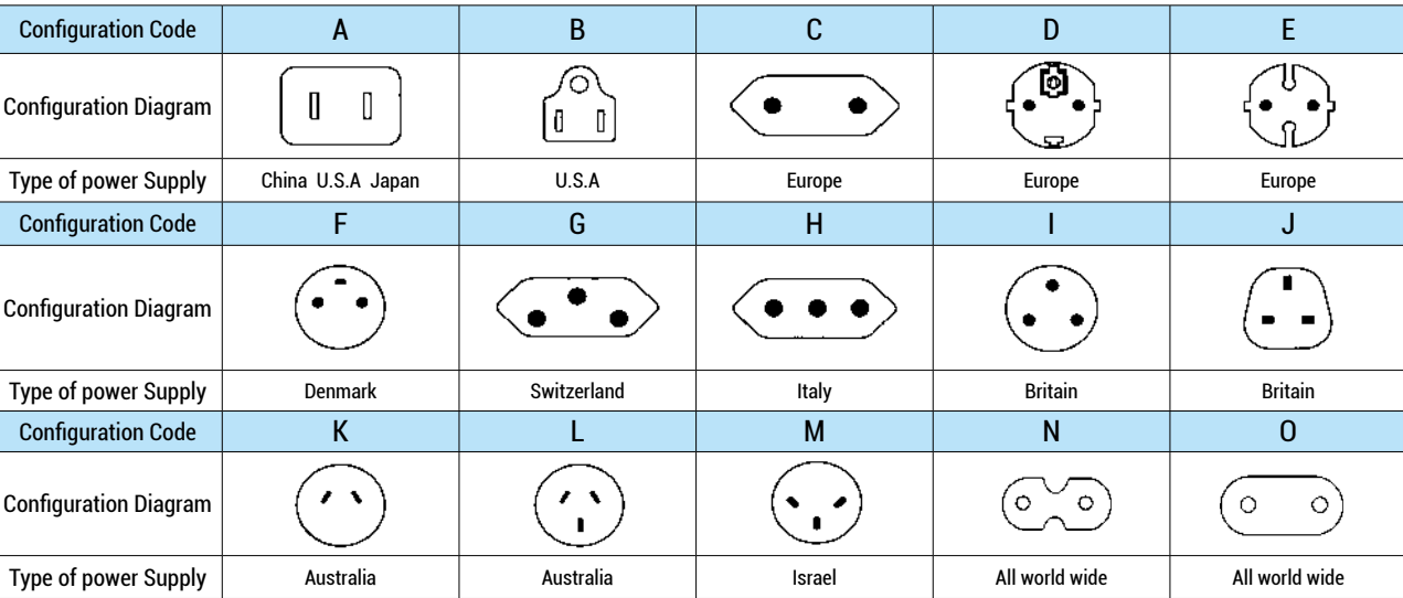
This chart presents an overview of power supply systems throughout the world. The configurations listed for the electrical systems of industrialized countries are accurate and reliable.
