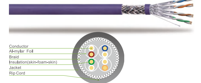
S/FTP Shielded CAT 6A Twisted Pair Installation Cable
