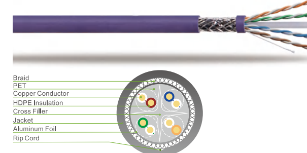
SF/UTP Double Fully Shielded CAT 6 Twisted Pair Installation Cable
