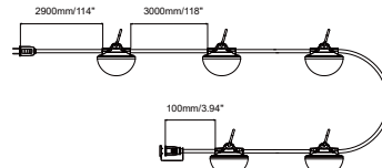
Option 1: It has 5 LED light heads and comes with a 50ft/ AC cord, Light heads spaced 10 feet/3mts apart
