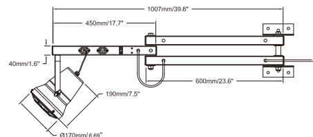
Double Arm with the 2 of receptacles
